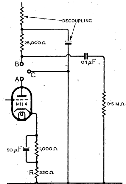
Fig. 3. A, B and C correspond to Fig. 1 and indicate the point of insertion of the filter in the amplifier.
