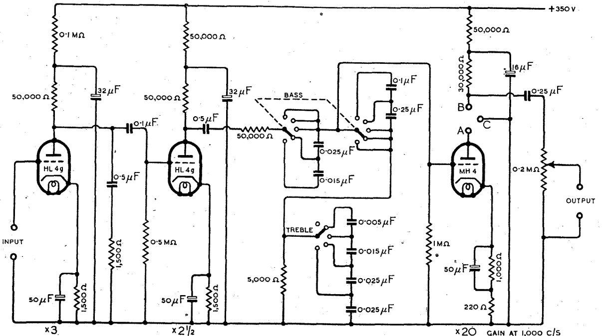
Fig. 7. Circuit diagram of complete gramophone feeder unit.
