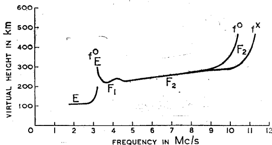
Fig. 2. Ionosphere characteristics: heights from which waves of various frequencies are returned under typical daytime conditions in winter.
