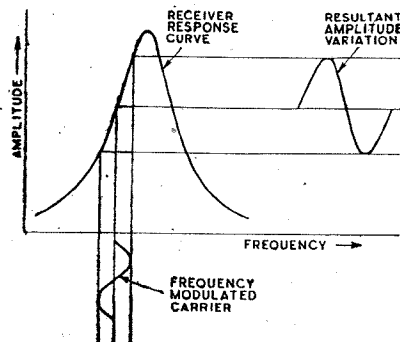
Fig. 7. The sloping side of the receiver response curve can be used to convert carrier frequency changes into variations of amplitude.
