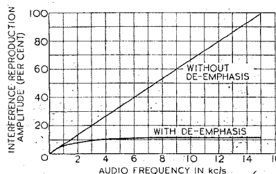
Fig. 3. Noise distribution over the audio band, with and without de-emphasis in a FM receiver.
