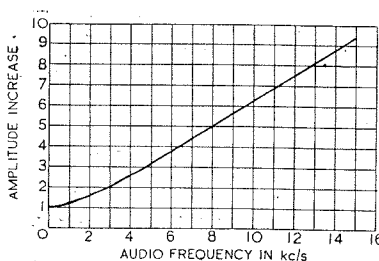
Fig. 2. American R.M.A. Television Transmission Standard (M9-218) for the pre-emphasis of high frequencies.
