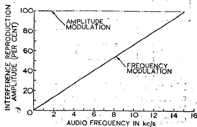
Fig. 1. Percentage amplitude at which noise is reproduced over the audio band with FM and AM transmission.
