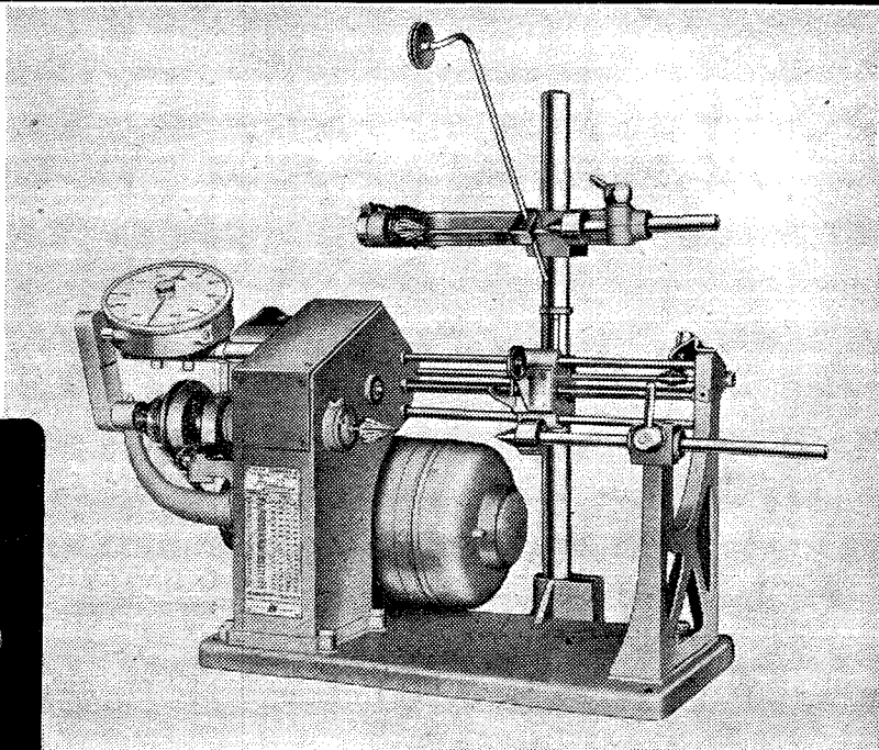
Model LW Coil Winding Machine
