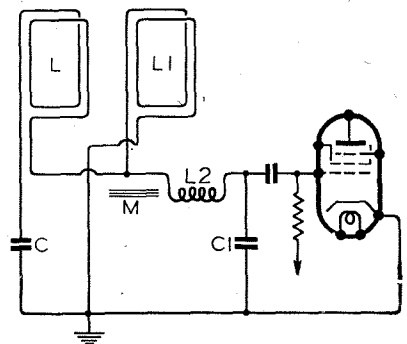
Constant coupling aerial circuit.
